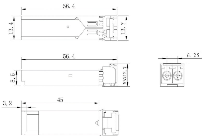
Outline Drawing
