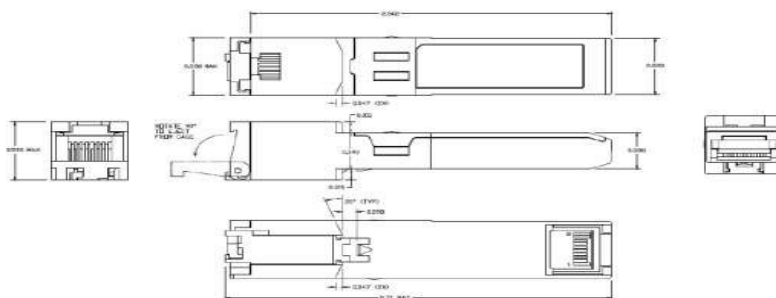
Figure 2. SFP-10/100/1000M-RJ45-100M mechanical dimensions
