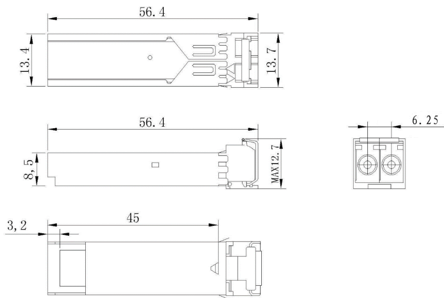
Outline Drawing
