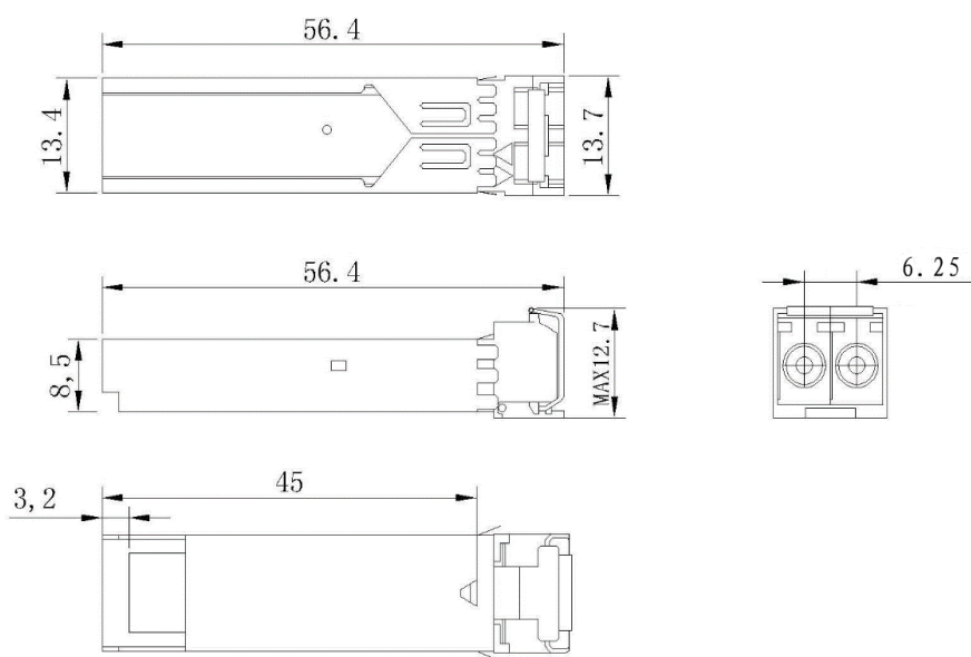
Outline Drawing
