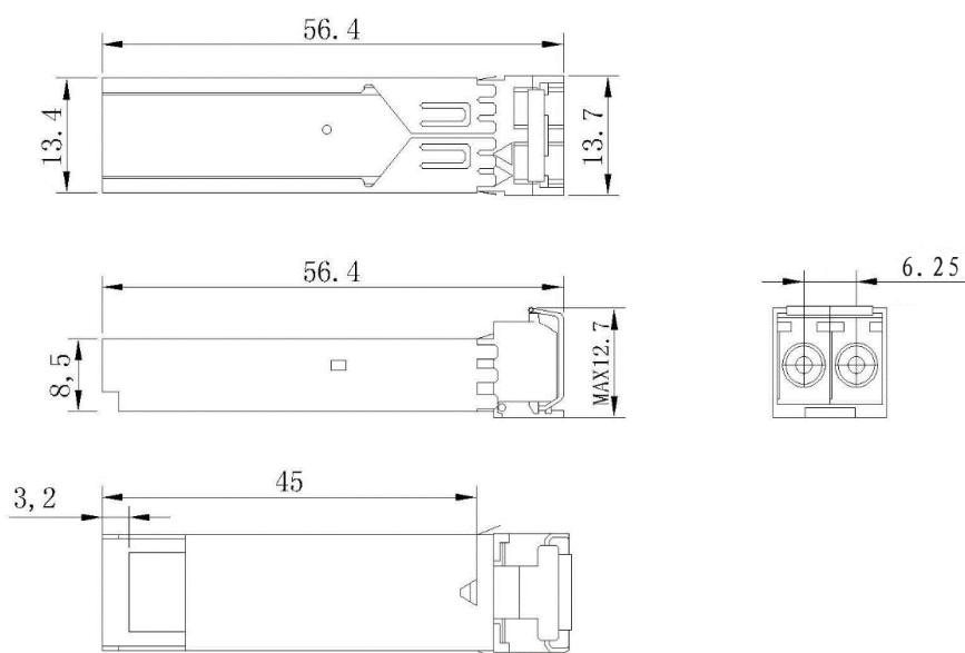
Outline Drawing
